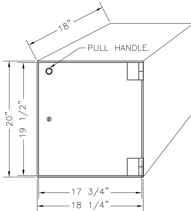
ELEVATION 1 COMPARTMENT LOCKER
